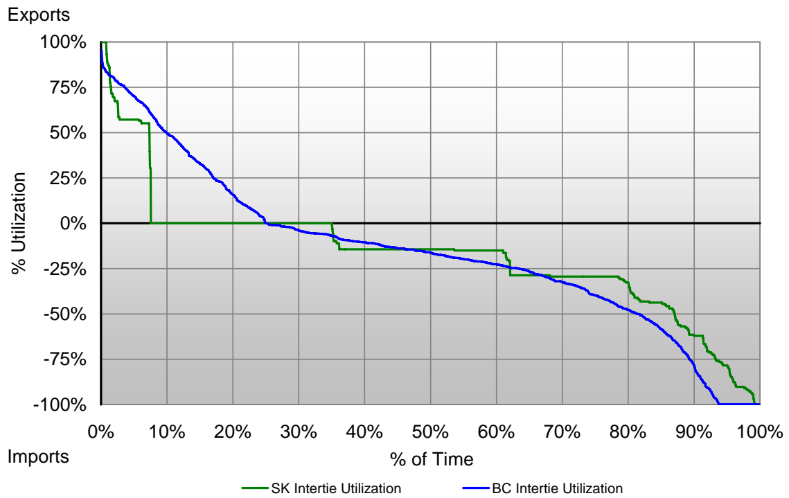
Figure 25 - Intertie Utilization
