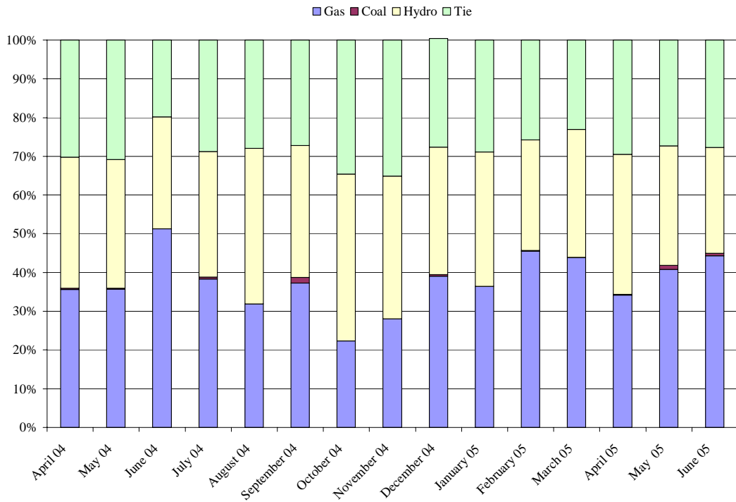
Figure 26 - Spinning Reserve Market Share by Fuel Type
