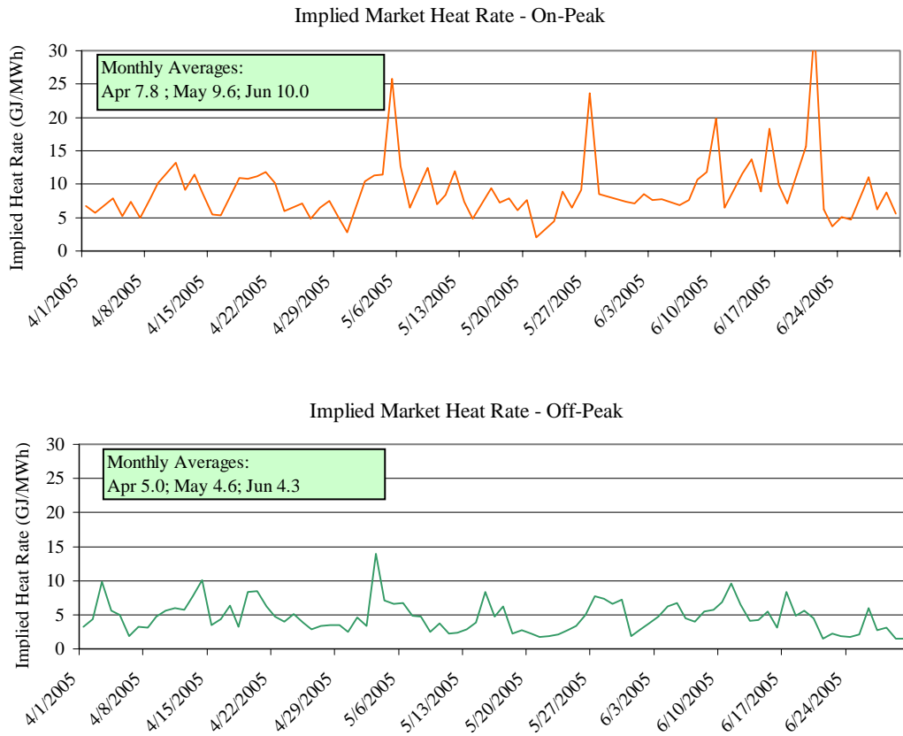
Figure 6 - Implied Market Heat Rates – Q2/05
