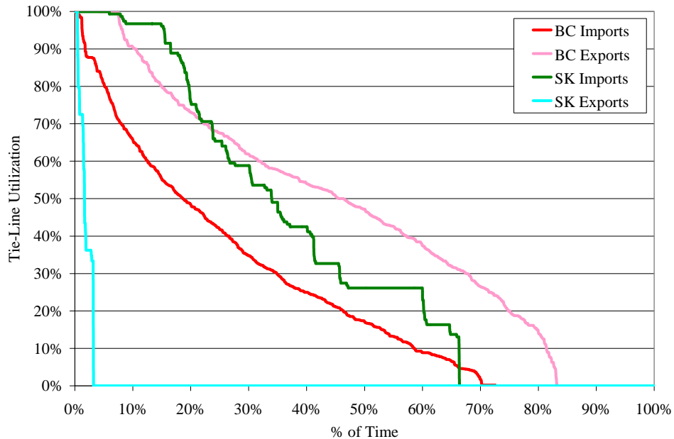
Figure 10 – Tie-Line Utilization, Q2/05
