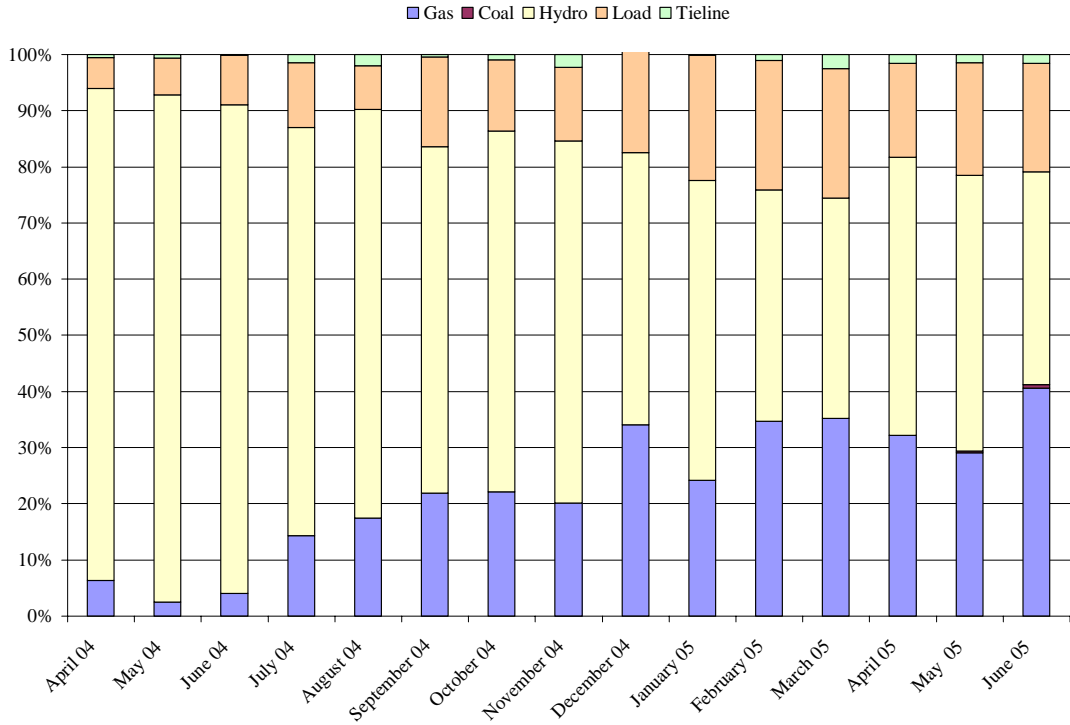
Figure 27 - Supplemental Reserve by Fuel Type
